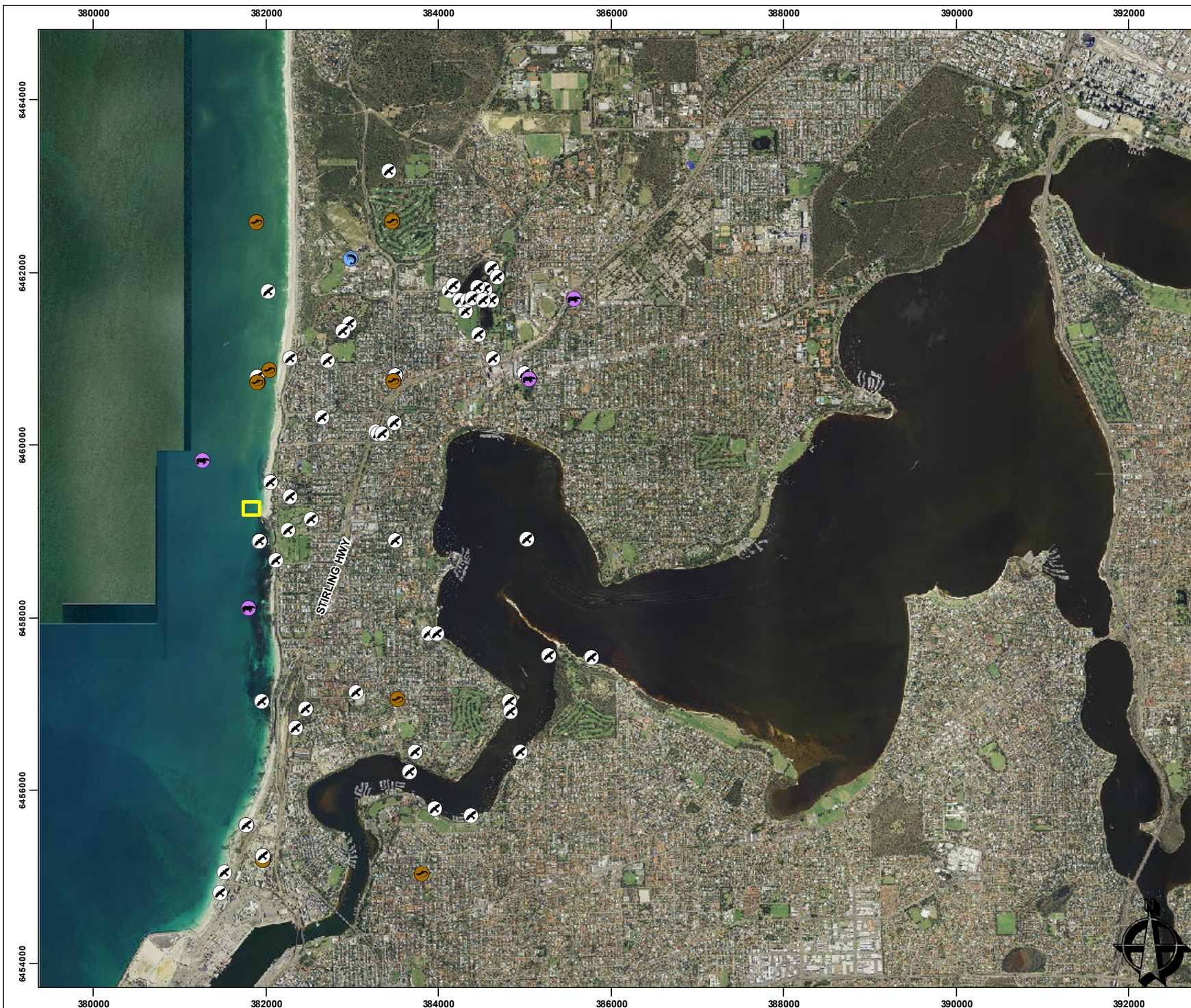
Figure 4 - Fauna
